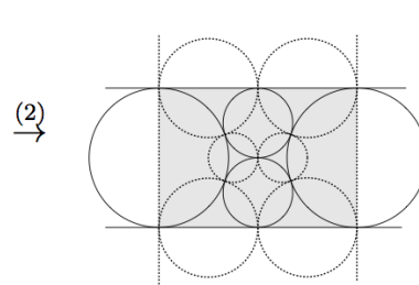
Figure 3: circle packing of a rectangle
